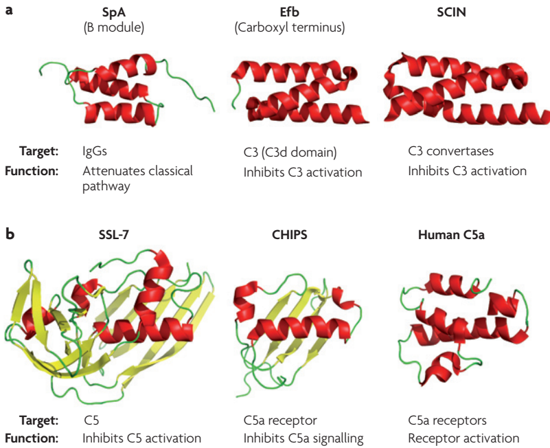
Figure 3 | Complement-targeting proteins in Staphylococcus aureus . A range of S. aureus proteins that interact with targets from the complement system have been structurally analysed. a | The immunoglobulin G (IgG)-binding module of staphylococcal protein A (SpA; Protein Data Bank (PDB) code: 1BDD 63 ), the C3-binding domain of the extracellular fibrinogen-binding protein (Efb; PDB code: 2GOM 74 ) and staphylococcal complement inhibitor (SCIN; PDB code: 2QFF 78 ) share similar structural motifs, but show differential functionality. b | Both staphylococcal superantigen-like protein-7 (SSL-7; PDB code: 1V1O 103 ) and the chemotaxis inhibitory protein of S. aureus (CHIPs; PDB code: 1XEE 104 ) attenuate complement on the level of C5, but bind to unrelated targets (C5 protein and C5a receptor, respectively). The solution structure of human C5a (obtained by nuclear magnetic resonance at pH 5.2; PDB code: 1KJS 105 ) is shown as a comparison. All protein-structure representations are coloured according to their secondary structure ( \alpha -helices in red and \beta -sheets in yellow).
