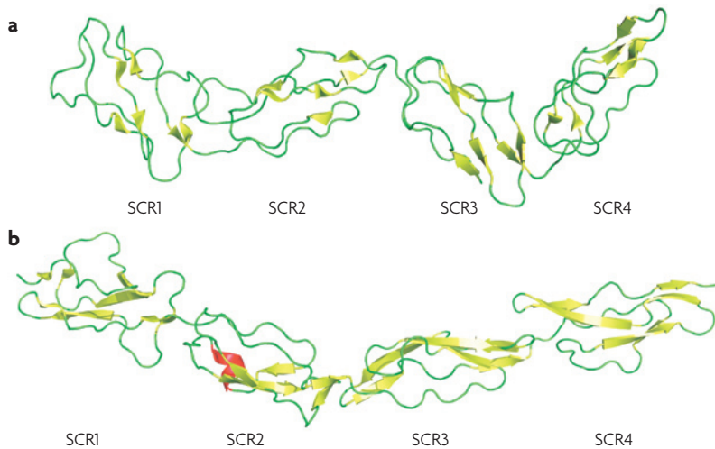
Figure 2 | Molecular mimicry of human complement regulators by viruses. Certain orthopox viruses and herpes viruses express proteins that closely mimic the structure and function of human regulators of complement activation. This structural similarity is illustrated for vaccinia virus complement-control protein (VCP; Protein Data Bank (PDB) code: 1G40 (REF. 27)) (a) and human decay-accelerating factor (DAF; PDB code: 1OJV 102 ) (b), both of which have four short consensus repeat (SCR) domains. These SCRs (or complement control protein modules) are common structural motifs in complement components (for example, complement receptors and regulators) and other proteins (such as selectins).
