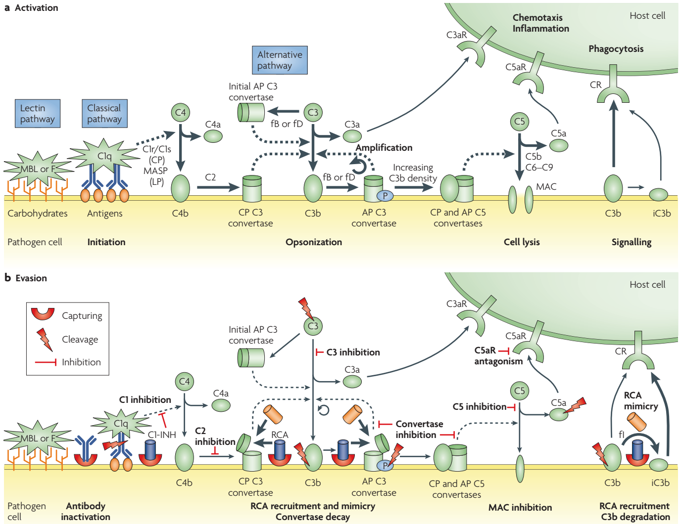
Figure 1 | Activation and evasion of complement. a | After activation of the complement system by antibody complexes (classical pathway (CP)), terminal mannose (lectin pathway (LP)) or by spontaneous and induced C3 hydrolysis (alternative pathway (AP)), the C3 convertases cleave C3 to its active fragments C3a and C3b. Covalent binding of C3b (opsonization) amplifies the cascade and mediates phagocytosis and adaptive immune responses by binding to complement receptors (CRs). Accumulation of deposited C3b also leads to the assembly of C5 convertases that activate C5 to C5a and C5b. Whereas C5b initiates the formation of the lytic membrane-attack complex (MAC), the anaphylatoxins C3a and C5a induce pro-inflammatory and chemotactic responses by binding to their receptors (C3aR and C5aR). On pathogenic surfaces, properdin (P) induces and stabilizes the AP C3 convertase, which leads to enhanced complement activity. b | Microorganisms have developed many ways to evade complement actions. Suppression of CP activation can be achieved by trapping endogenous C1 inhibitor (C1-INH) to the surface or by inactivating antibodies through the capture of their Fc regions. Whereas the recruitment of soluble regulators by capturing host proteins is a common strategy to impair downstream complement actions, certain viruses also produce structural mimics of these regulators. In addition, some microbial proteins have similar activities to CD59 in preventing MAC formation. Direct inhibition of C3, the C3 and C5 convertases, C5 or the C5a receptor (C5aR) is a prominent strategy of Staphylococcus aureus . Finally, a set of different microbial proteases can degrade many of the crucial components of the complement system. These proteases act directly or by capturing and activating a human protease. An extended list of complement evasion proteins can be found in Supplementary information S1 (table). Increased and decreased activity is represented by thick and thin arrows, respectively. F, ficolin; fB, factor B; fD, factor D; fI, factor I; MASP, MBL-associated serine protease; MBL, mannose-binding lectin; RCA, regulators of complement activation.
